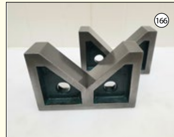
PRECISION VEE BLOCKS: Overall Height 6". Length Across Vee's 7". £325
