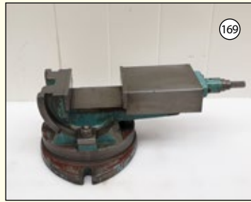
ABWOOD: Tilting, Turning Machine Vice. Max Jaw Opening 5". Jaw Width 6 1/4". £450
