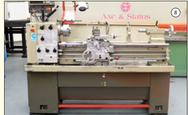
HARRISON M300: Gap Bed Centre Lathe. Swing Over Bed 13". Distance Between Centres 40". Speeds 40-2500rpm. 3 & 4 Jaw Chucks. QCTP. 2 Axis DRO.
