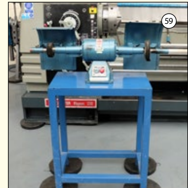
RJH GRYPHON: Polishing Machine. Max Wheel Speed 3000rpm. 240 Volt. £650
