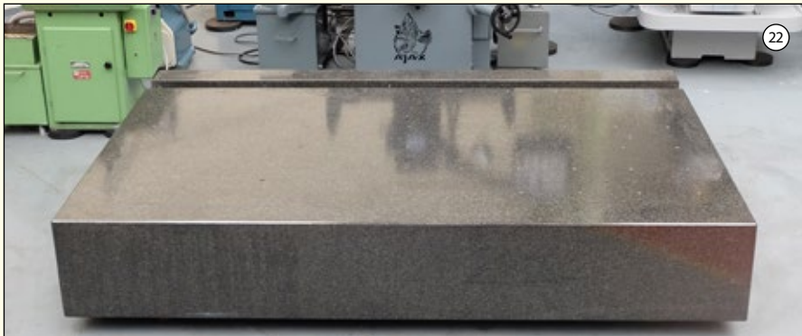
GRANITE SURFACE TABLE: Ex Coordinate Measuring Table. Total Table Size 2860mm x 1880mm. Thickness 460mm. Main Table Without Cut-Out 2860mm x 1590mm. £2,250
