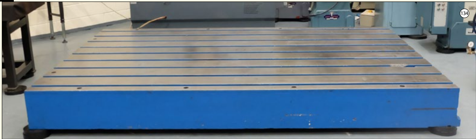
TEE SLOTTED: Cast Iron Floor Plate. Size 12' x 7' 8" x 14" Thickness.
