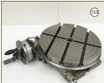
TEE SLOTTED ROTARY TABLE: With Dividing. 380mm Diameter. 120mm Height.
