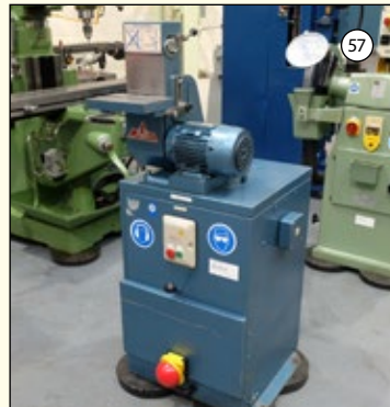
RJH: Vertical Bandfacer on Dust Extractor. Belt Size 100mm x 915mm. Motor 0.75kw. 3 Phase 415V. £1,250
