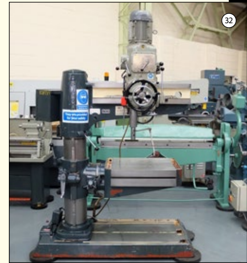
RICHMOND Type SR2: 3' Radial Arm Drill. Spindle Taper 3MT. Speeds 50-1500rpm. Drilling Cap 1". Power Feed to Spindle. Table 29" x 21". DC Brake. £3,950
