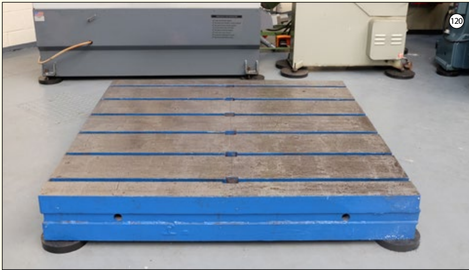
TEE SLOTTED: Floor Plate: Size 6' x 6' x 10" Thickness. 6 x Tee Slots.
