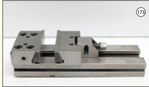
MODULAR GROUND VICE: Max Opening 200mm. Jaw Width 150mm. Overall Height 100mm. £375
