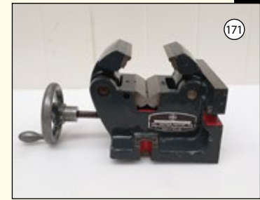
ELLIOTT: Self Centering Pipe Vice. Width of Jaws 4 3/8". Opening of Jaws 3 1/8". £425
