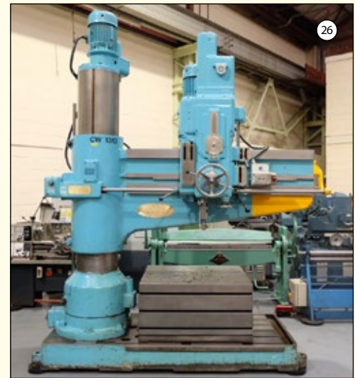
KITCHEN & WADE Type E27: 6' Radial Arm Drill. Arm Radius 72". Drilling Cap 3". 5MT. Speeds 8.5-800rpm. Drilling Depth 18". Box Table 42" x 36" x 22" High. Telescopic Brake. £6,950
