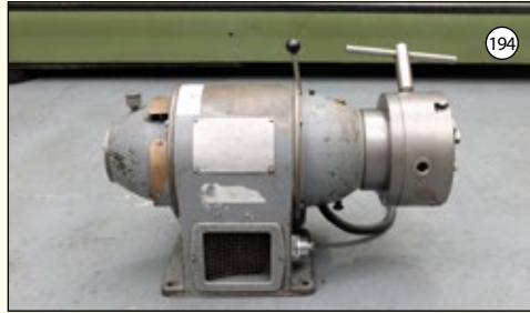
MOTORISED WORKHEAD: 3 Jaw Chuck 160mm. 14" Swing. 2 Speed.
