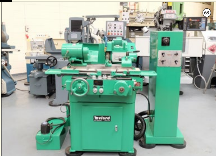
MYFORD MG12-HA: Hydraulic Cylindrical Grinder. Maximum Grinding Capacity 3" Diameter. Swing Over Table 5". Max Table Travel 13 3 / 4 ". Capacity Between Centres 12".
