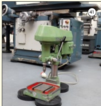
FLOTT Type TB6: High Speed Bench Drill. Throat 6 1/2". Capacity 1/4". Tee Slotted Base 12" x 9". Speeds 450 - 9000rpm. £475
