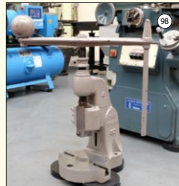
DENBIGH No4: Fly Press. Throat 4 1 / 2 ". Daylight 7 1 / 2 ". Approx Tonnage 4.
