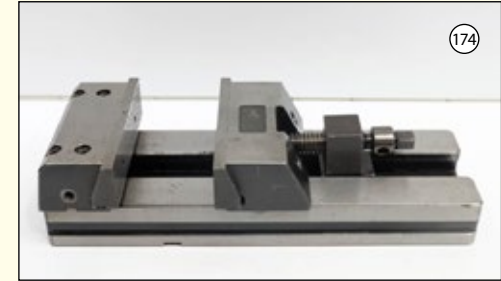
MODULAR GROUND VICE: Max Opening 250mm. Jaw Width 200mm. Overall Height 135mm. £475
