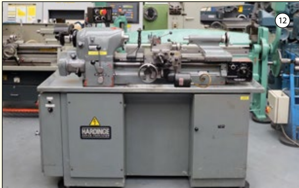
HARDINGE Model HLV-H: High Precision Centre Lathe. Swing Over Bed 11". Distance Between Centres 18". Variable Speed 125 - 3000rpm. Metric Gearbox. With 3 & 4 Jaw Chucks. Face Plate. 3 Point Steady. Drawbar & Collets. £8,750
