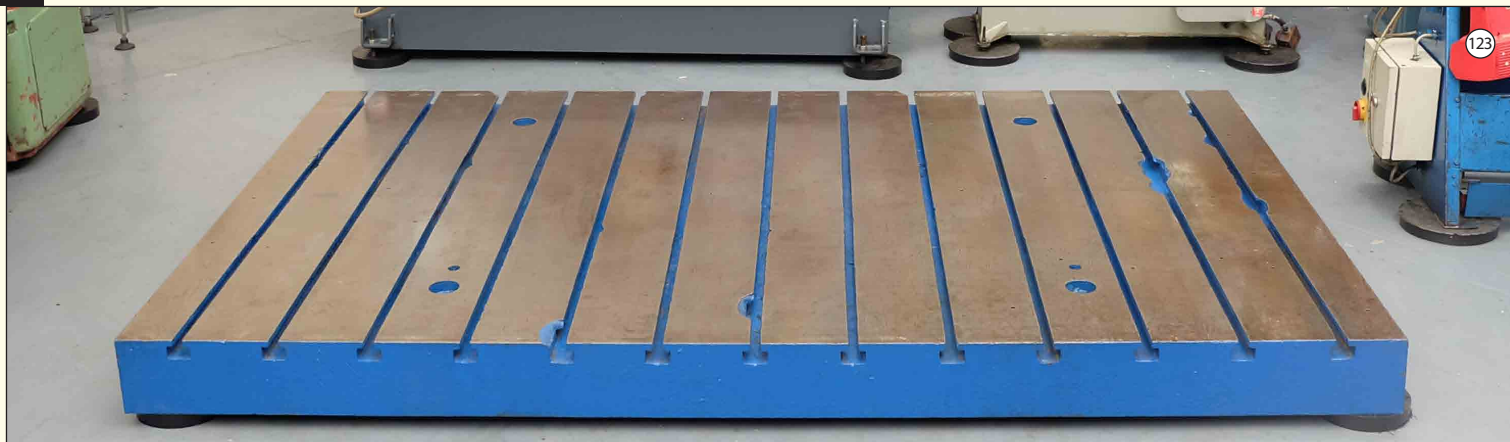
TEE SLOTTED: Floor Plate. Size 10' x 6' x 8" Thickness. 13 x Tee Slots.
