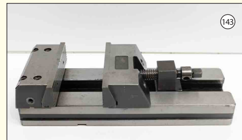
MODULAR GROUND VICE: Max Opening 250mm. Jaw Width 200mm. Overall Height 135mm. £475
