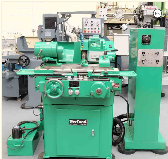
MYFORD MG12-HA: Hydraulic Cylindrical Grinder. Maximum Grinding Capacity 3" Diameter. Swing Over Table 5". Max Table Travel 13 3 / 4 ". Capacity Between Centres 12".
