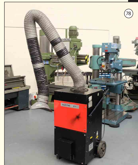
ELECTAC Model E1: Mobile Welding Fume Extractor/Filter. Articulated Suction Boom 2.5 Mtr. 750 Watts. 115 Volts.
