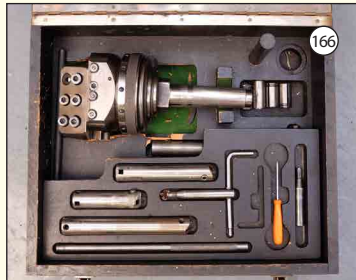
WOHLHAUPER UPA4/13015: Universal Boring & Facing Head. 4MT. 14mm Thread.
