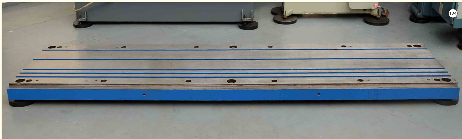
TEE SLOTTED: Floor Plate: Size 146" x 35" x 5" Thickness. 5 x Tee Slots.
