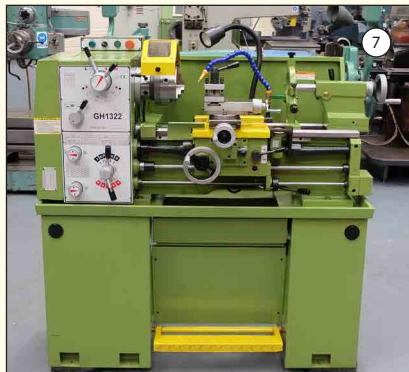
WARCO Model GH 1322: Gap Bed Centre Lathe. Swing Over Bed 330mm. Speeds 70-2000rpm. Between Centres 500mm. 2&3 Point Steadies.
