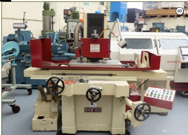
XYZ Type 1632: Toolroom Surface Grinder. Capacity 32" x 16". Distance Spindle Centre to Table 22" Max. Wheel Size 16" x 2" x 5" Bore. Wheel Speed 1500rpm. Power Rise & Fall to Spindle Head. Electro Mag Chuck 32" x 16". Coolant Tank & Wheel Balance Unit. £14,250
